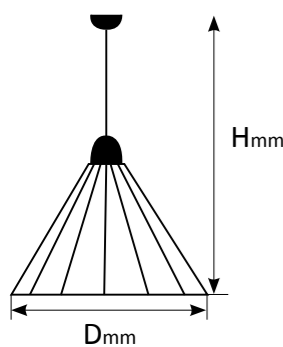
LS 3120-115-1L E27 1x60 D = 115 H = 750
